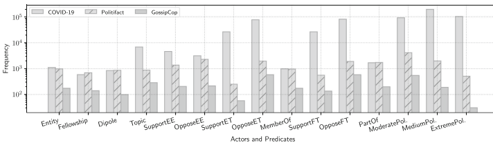
Fig. 5. Frequency of PKG actors and predicates. ModeratePol. , MediumPol. , and ExtremePol. represent Has[Moderate, Medium, Extreme]Polarization predicates.
